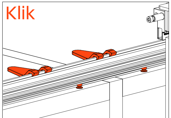
Guide tracks installed with press-fit clips.
