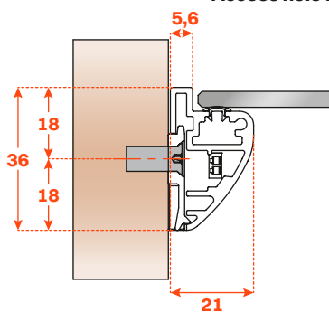
Front profile with LED
