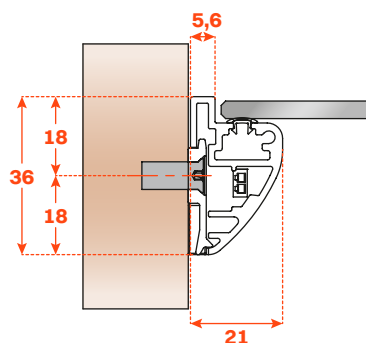
Perfil frontal com LED
