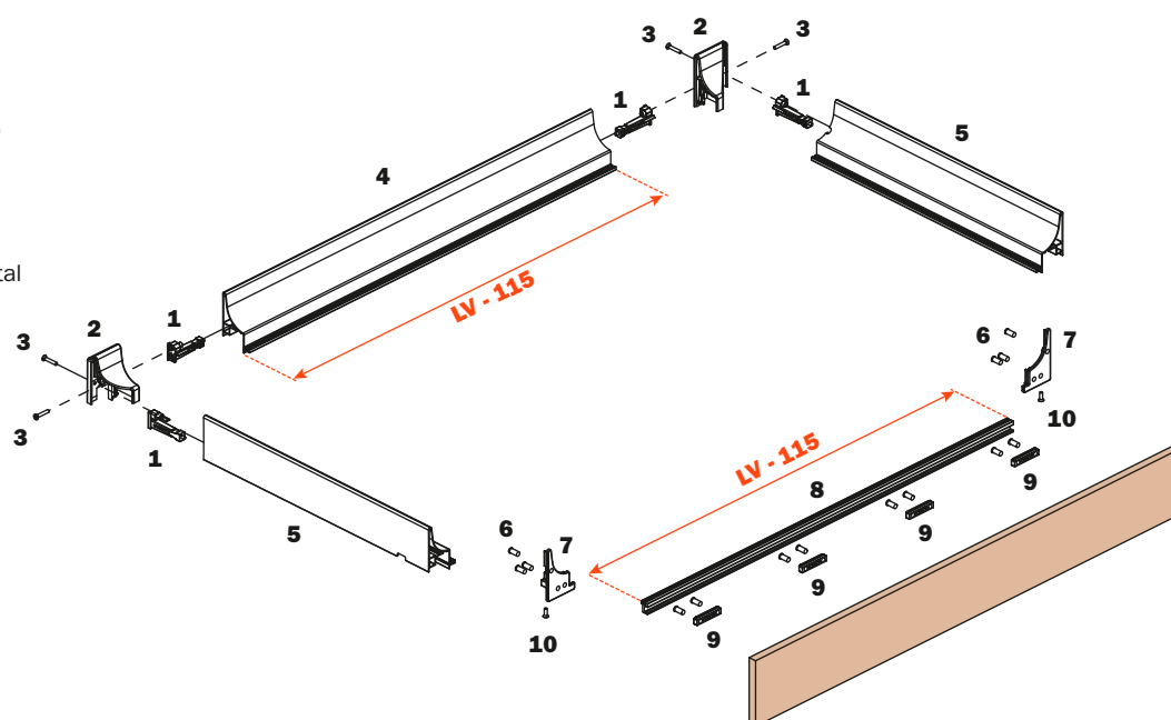
PART NUMBER KIT RUNNERS AND SIDE PROFILES Runner length (LN) mm Drawer depth (P) mm PACKAGE DIMENSIONS mm PACKAGE WEIGHT Kg VE80QDAG40033A 400 440 121 x 681 x H 116 3 VE80QDAG45033A 450 490 121 x 731 x H 116 3.4 VE80QDAG47033A 470 510 121 x 751 x H 116 3.7
