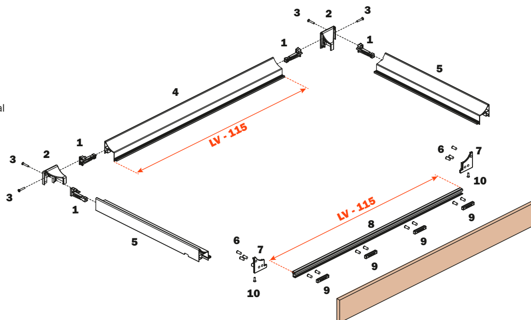
PART NUMBER KIT RUNNERS AND SIDE PROFILES Runner length (LN) mm Drawer depth (P) mm PACKAGE DIMENSIONS mm PACKAGE WEIGHT Kg VE80QBAG40033A 400 440 121 x 681 x H 116 2.8 VE80QBAG45033A 450 490 121 x 731 x H 116 3.2 VE80QBAG47033A 470 510 121 x 751 x H 116 3.4
