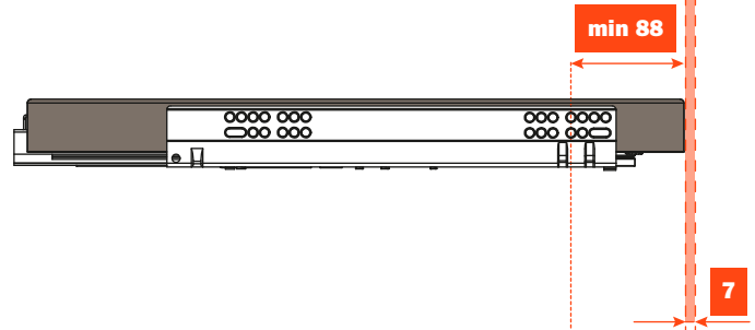
3-SIDED drawer for wood front, 19 mm thickness
