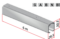
2201 Aluminium-Schiene
