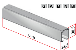
2201 Aluminium-Schiene
